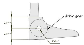
Dimensioned View
